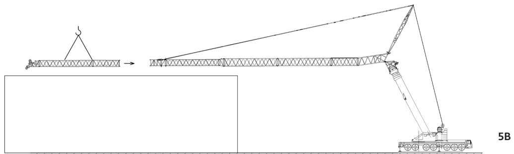
Rigging on obstacles
